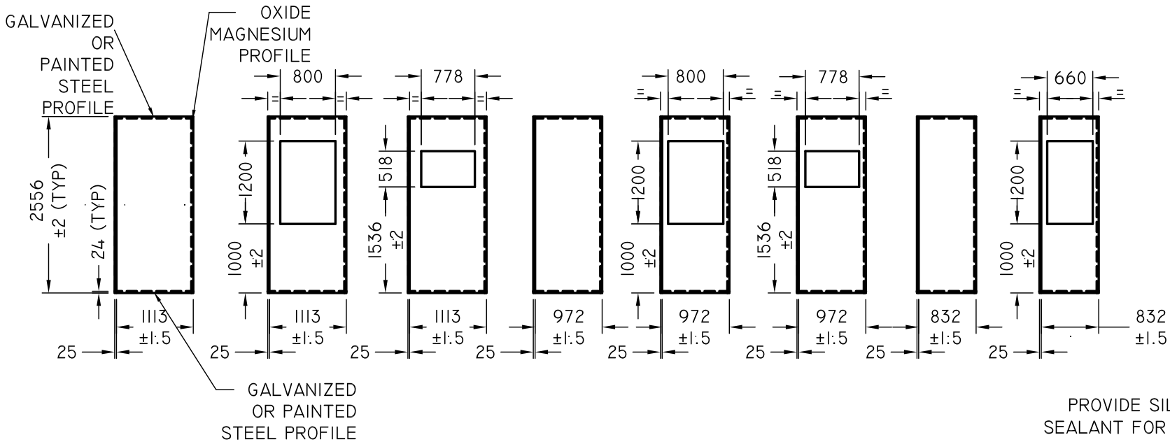
WALL PANEL TYPE OPENINGS
