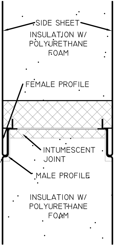
PANEL MATEUP DETAIL
